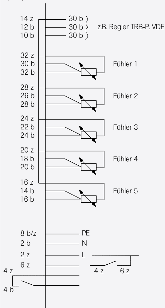
Pin assignment z and d
